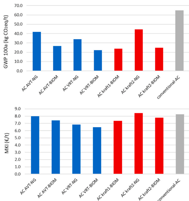
Fig. 10. Comparing the cradle-to-grave impacts of 1 t of top-layer asphalt using biorefinery lignins (blue) using kraft lignins (red) and conventional asphalt (grey). Top graph for climate change. Bottom graph for MKI score (bottom).
